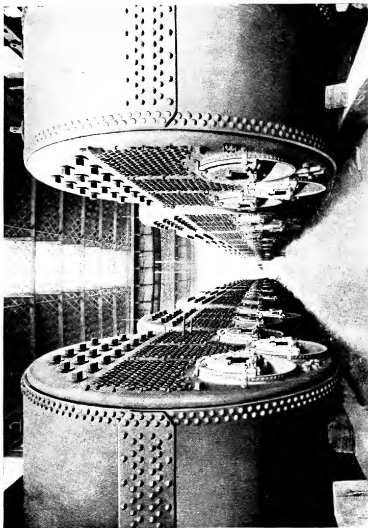
BOILERS OF THE TITANIC ARRANGED IN MESSRS. HARLAND & WOLFF'S WORKS
